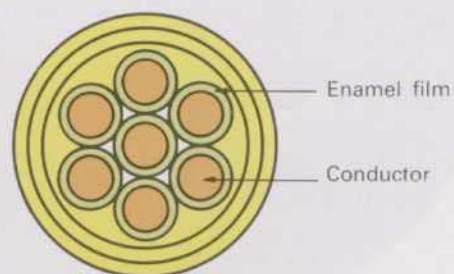
C: Litz wire type (TEX-ELZ)
